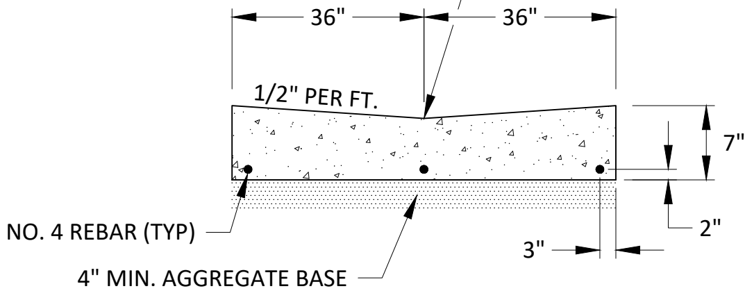
SECTION A-A THRU CONCRETE GUTTER
