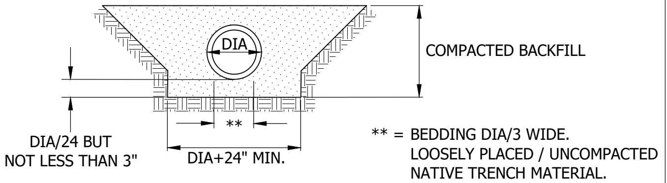
INSTALLATION TYPE 3
